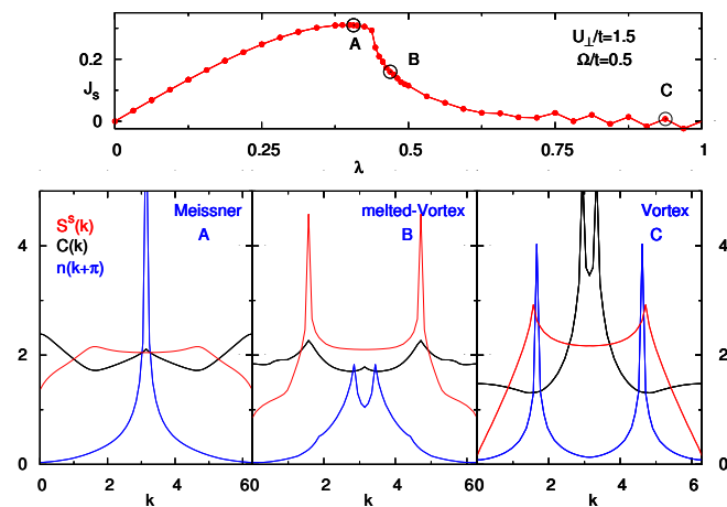
FIG. 7. Upper panel shows the spin current J_s as a function of the applied flux, red line is only a guide to eye. Panels below show S^s(k) (red solid line), C(k) (black line), n_\sigma(k) (blue line) where the argument of this last quantity has been shifted of \pi . Left, center and right panels show these quantities for the cases indicated by the point A , B and C in the upper panel, respectively corresponding to cases where the system is in the Meissner phase, in the melted-Vortex phase and in the Vortex phase. Data shown are from DMRG simulations in PBC for L=64 . Color online.
