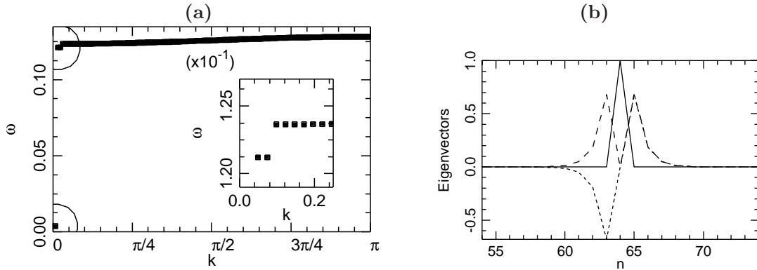
Fig. 19. (a) Linear spectrum of the equilibrium solution shown in Fig. 18 for the case K = 0.00045 eV \text{\AA}^{-2} . The circles attract the attention on three particular frequencies which are outside of the phonon band. One of them is far below the band. It is the frequency \omega_b of the discrete breather. The two others also correspond to localized modes. The inset shows a magnification of the lower k part of the phonon band. The two frequencies right below the band are clearly visible. (b) Plot of the eigenvectors associated with the three modes which are outside of the phonon spectrum. The full line corresponds to the lowest mode, and, as expected it has the shape on the discrete breather. The dotted line corresponds to mode 2 and the dash line to mode 3.
