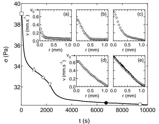
FIG. 2: The shear-stress \sigma vs time t for a shear rate \dot{\gamma} = 0.7 s ^{-1} applied at t = 0 . Insets: velocity profiles v(r) , where r is the distance to the rotor, at different times [symbol, time (s)]: ( \square , 27); ( \triangle , 1013); ( \diamond , 1730); ( \nabla , 2250); ( \bullet , 6778); ( \circ , 9413). The arrow indicates the rotor velocity v_0 . Both walls have a roughness of 60 \mu m. The two-step relaxation of \sigma(t) is strongly correlated to the evolution of v(r) (see text).
