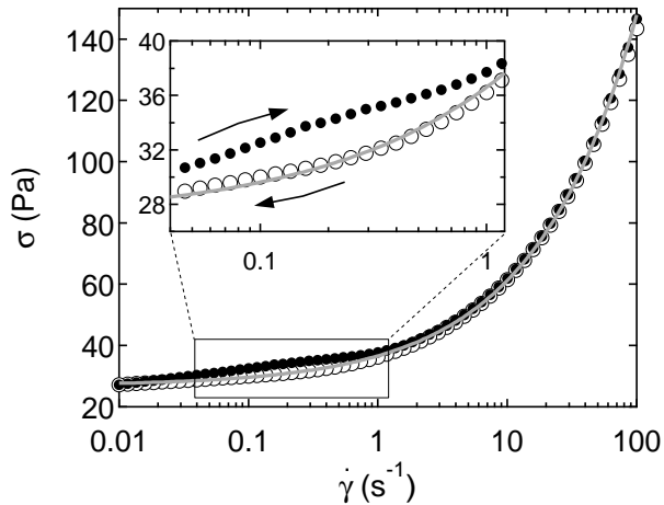
FIG. 1: The flow curve, shear stress \sigma vs the shear rate \dot{\gamma} , obtained by decreasing \dot{\gamma} from 100 to 0.01 s ^{-1} ( \circ ) and then increasing \dot{\gamma} from 0.01 to 100 s ^{-1} ( \bullet ) with a waiting time of 100 s per point. Note the slight hysteresis for \dot{\gamma} \lesssim 1 s ^{-1} which is the signature of a significant slowing down of the system dynamics near the yielding transition (see text). The gray line is the best fit of the decreasing part by the Herschel-Bulkley model: \sigma = \sigma_c + A\dot{\gamma}^n , with \sigma_c = 26.9 Pa, n = 0.55 and A = 9.8 Pa.s ^{-n} . Inset: zoom over the low shear rate regime. Both walls have a roughness of 60 \mu m.
