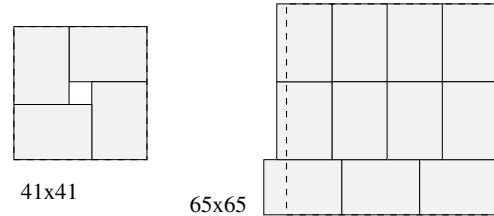
Figure 4: Tilings for 41x41 and 65x65 multiplications.
