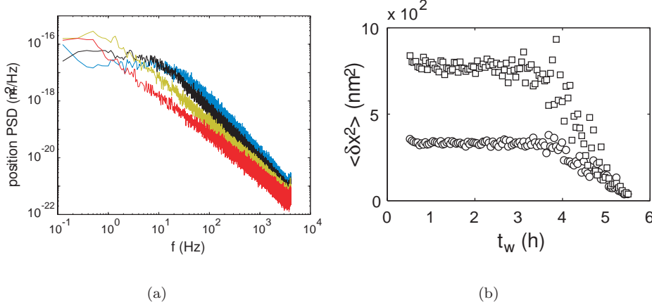
Figure 3: (a) Spectra of the particle position fluctuations inside a Laponite solution at 2.3% wt. The spectra has been measured for the trap stiffness k_1 = 6.34 \text{ pN}/\mu\text{m} at various ageing times: from right to left t_w = 30, 110, 190 and 270 minutes. (b) Evolution of \langle \delta x^2 \rangle with t_w for both stiffness, k_1 = 6.34 \text{ pN}/\mu\text{m} ( \square ) and k_2 = 14.4 \text{ pN}/\mu\text{m} , ( \circ ). The variances have been measured on a time window of \tau = 61 \text{ s} .
