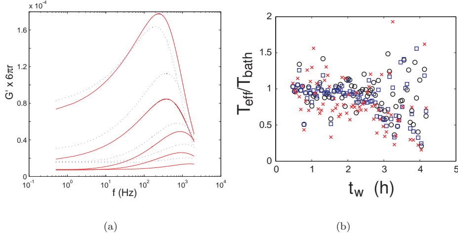
Figure 7: (a) Evolution of 6\pi r G' (the global elastic modulus) as a function of frequency for both trap stiffnesses, k_1 = 7.47 \text{ pN}/\mu\text{m} (solid lines), k_2 = 16.7 \text{ pN}/\mu\text{m} (dashed lines) and for increasing aging time: t_w = 30 \text{ min} , 90 \text{ min} , 140 \text{ min} , 190 \text{ min} and 240 \text{ min} (1.2% wt of Laponite, 2 \mu\text{m} glass bead and ionic strength I = 5 \times 10^{-3} \text{ mol l}^{-1} ). (b) Evolution of the ration T_{eff}/T_{bath} with aging time ( t_w ) for different frequencies ( f = 1 \text{ Hz} \square , 10 \text{ Hz} \circ and 100 \text{ Hz} \times )).
