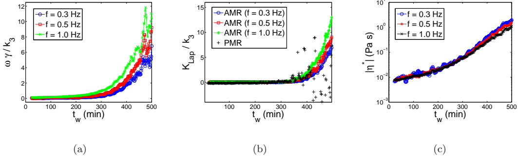
Figure 8: (a) Time evolution of viscosity of the colloidal glass obtained by means of AMR. (b) Time evolution of elasticity of the colloidal glass obtained either by PMR and AMR. (c) Time evolution of the modulus of the complex viscosity
