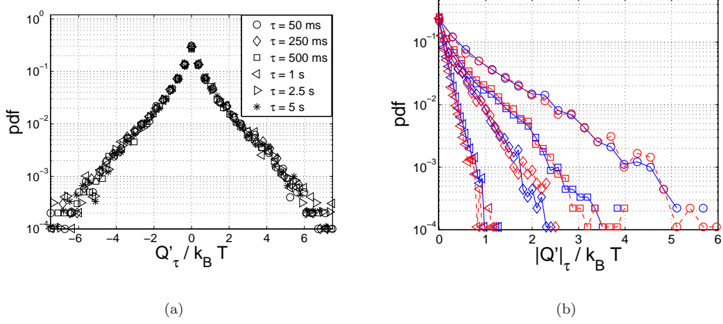
Figure 11: (a) PDFs of Q'_\tau at t_w = 95 min for different values of \tau . (b) PDFs of |Q'_\tau| for \tau = 5 s at different aging times t_w after the onset of gelation (from top to bottom: t_w = 340, 435, 470 and 500 min). Blue points correspond to Q'_\tau > 0 while red ones to Q'_\tau < 0 .
