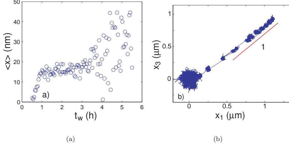
Figure 5: (a) Evolution of the mean position along the x -direction with aging time, same data as in Fig. 3. (b) Comparison of the trajectories for two 1\mu\text{m} in diameter glass beads of whose fixed traps are separated by 6.5\mu\text{m} during the evolution of the suspension of Laponite ( I = 5 \times 10^{-3} \text{ mol l}^{-1} , 1.2% wt of Laponite). Each pincushion represents 1 second of measurement at 288 Hz, repeated every 5 min during 150 min.
