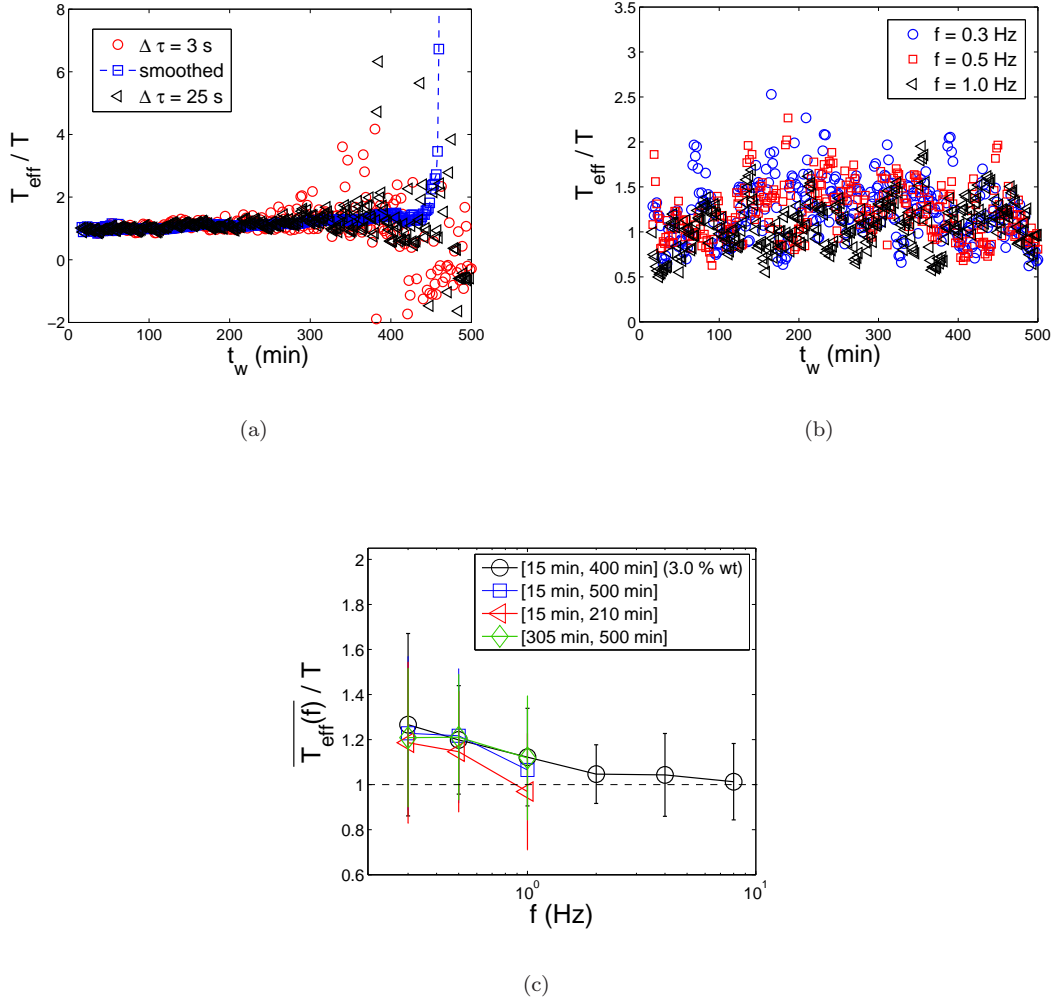
Figure 10: (a) Time evolution of effective temperatures of the colloid during aging obtained by means of PMR (see text for symbols). (b) Time evolution of effective temperatures for different frequencies obtained by means of AMR. (c) Aging time average of the effective temperatures obtained by AMR for different frequencies. Error bars represent the standard deviation of data shown in Fig. 10(b).
