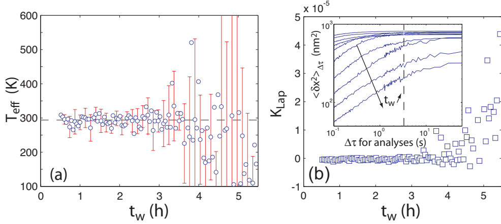
Figure 4: (a) Evolution of the effective temperature with aging time for the data of Fig. 3 k_1 = 6.34 \text{ pN}/\mu\text{m} , k_2 = 14.4 \text{ pN}/\mu\text{m} , 2.3% wt of Laponite and r = 1 \mu\text{m} glass bead. The error bars are computed from the statistical error of \langle \delta x_j^2 \rangle at the time t_w . (b) Evolution of the stiffness of the Laponite with ageing time. Inset: Evolution of \langle \delta x^2 \rangle_{\Delta\tau} for k_1 = 6.34 \text{ pN}/\mu\text{m} as a function of the duration \Delta\tau of the samples for different aging times : t_w = 30, 57, 83, 110, 137, 163, 190, 217, 243 and 270 minutes.
