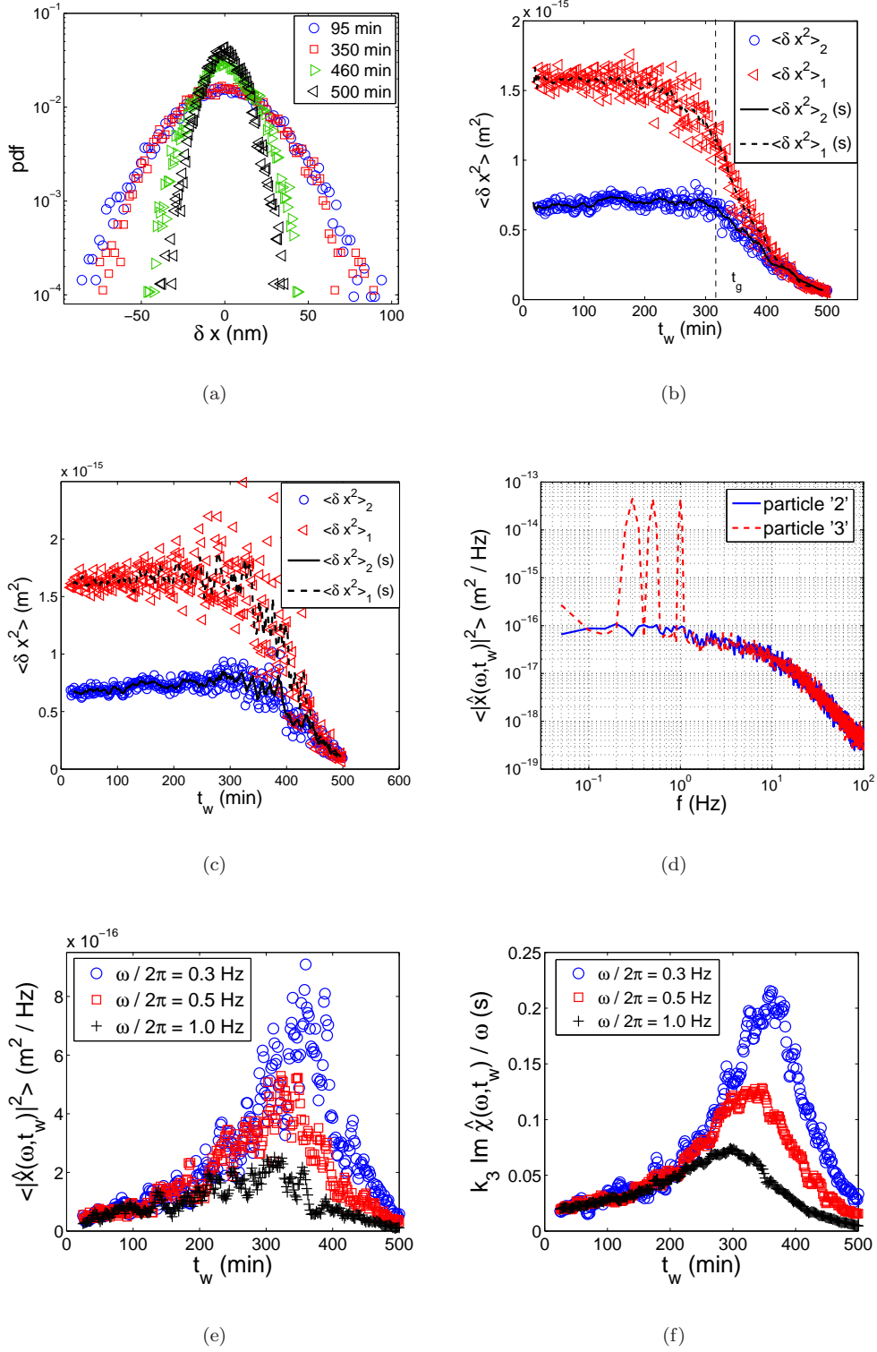
Figure 9: (a) PDFs of \delta x at different t_w for particle '2'. (b) Time evolution of variances for particles '1' and '2' computed for \Delta\tau = 3 s. The thin dashed line indicates the approximate aging time when gelation begins to take place. Labels (s) correspond to smooth curves (see text). (c) Time evolution of variances computed for \Delta\tau = 25 s. (d) Spectra of displacement fluctuations of particles '2' and '3' at t_w = 95 min. (e) Time evolution of the power spectral densities of displacement fluctuations of particle '2' for the three frequencies studied. (f) Time evolution of the imaginary part of the Fourier transform of the response functions of particle '3'.
