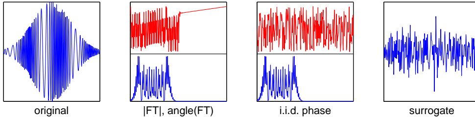
Figure 1. Surrogate. From left to right: original signal, its Fourier transform (top: phase, bottom: magnitude), same after phase randomization, the surrogate.
