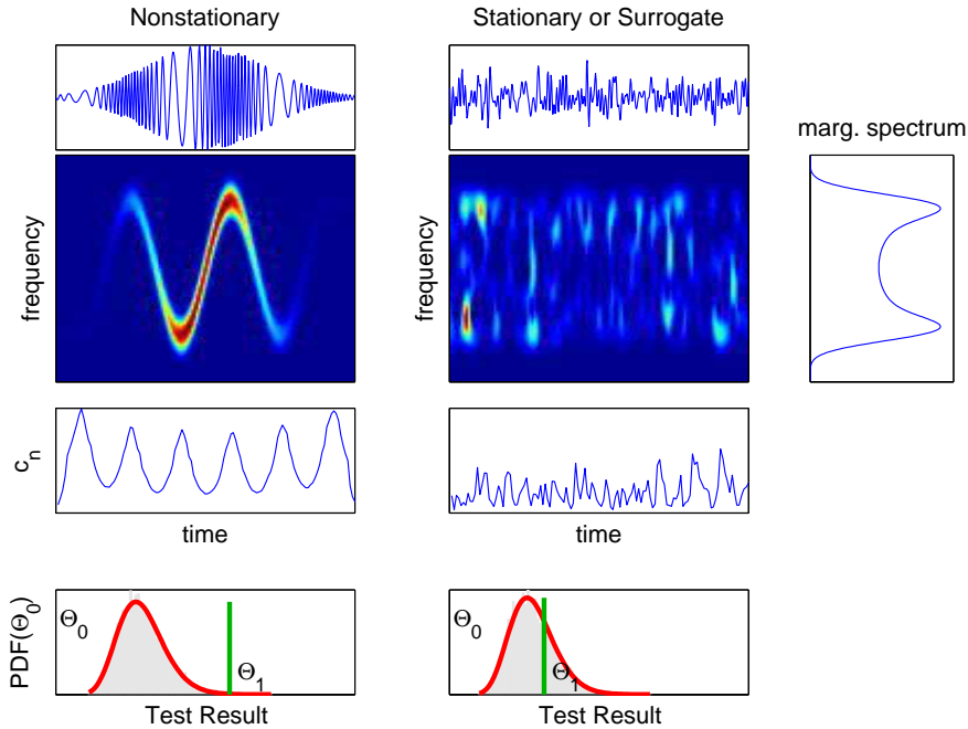
Figure 3. Stationarity Test. From top to bottom: signal, multitaper spectrogram, local contrast c_n , and statistics of the test. Left: original (nonstationary) signal; Right: stationary surrogate. Last row: the distribution of \Theta_0(j) is displayed in gray (fitted with a Gamma law [13]). One sees that \Theta_1 (the green line) is an outlier for the distribution on the left, and is inside the distribution for a stationary signal (on the right). Parameters: K = 5 , J = 50 .
