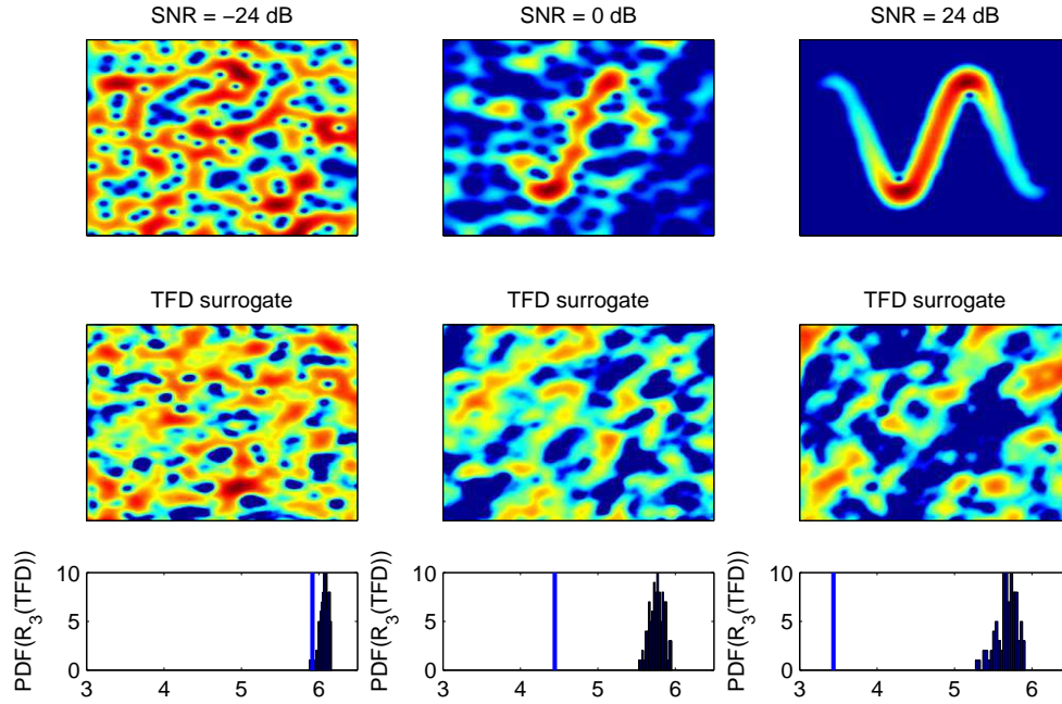
Figure 5. Transient Detection. The detection test is applied to a chirp embedded in a white Gaussian noise with several SNR (-24, 0 and 24 dB). From top to bottom: TFD of the signal with noise, TFD surrogate with positivity constraint; statistics for the test (Rényi entropy of order 3): (blue) vertical bar for the signal, (black) histogram for the surrogates.
