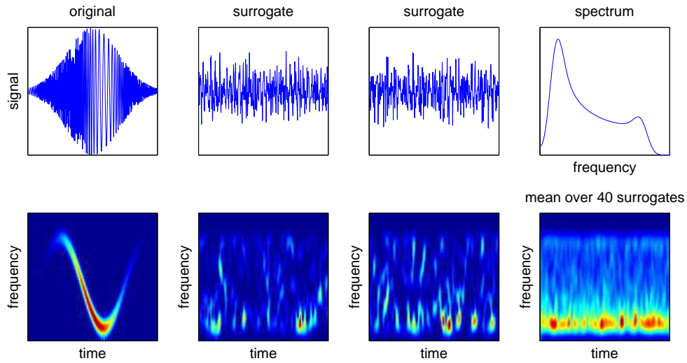
Figure 2. Surrogates in time-frequency domains. Top: A nonstationary signal and two representative surrogates, with their common time-averaged spectrum on the far right. Bottom: multitaper spectrogram of the signals. One sees that for surrogates, structures are destroyed and one recovers a time-varying spectrum that fluctuates around the mean stationary spectrum (displayed on the right). Spectrograms are color-coded (red is large values, blue is zero). Parameters: K = 5 ; 512 points in time and frequency.
