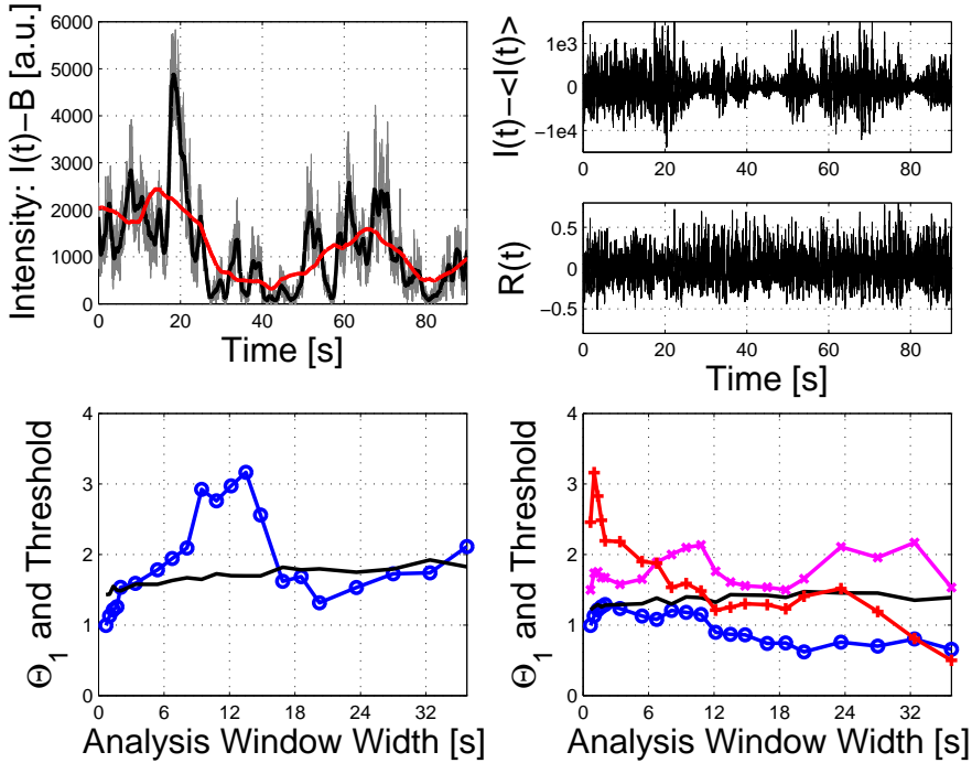
Figure 4. Test of stationarity of dynamic light scattering. Data from [26]: SHEP cell in the G1 phase; acquisition frequency is 10^3 Hz. Top left: raw scattering intensity and moving average \langle I(t) \rangle_T of the signal for T = 1 s (black) and 15s (red) (baseline B_0 removed). Bottom Left: Result of the stationarity test for I(t) according to window width (threshold \gamma for stationarity in black; test statistics \Theta_1 in blue). Top right: Fluctuations I(t) - \langle I(t) \rangle_T , and (renormalized) fluctuations R(t) (for B_0 here). Bottom right: Result of the stationarity test for R(t) (threshold in black), for different fixed baseline B (red: B_0 - 600 , blue: B_0 , or magenta: B_0 + 300 ). Only with the correct one, B_0 , the test validates that the fluctuation is stationary for almost all analysis scales.
