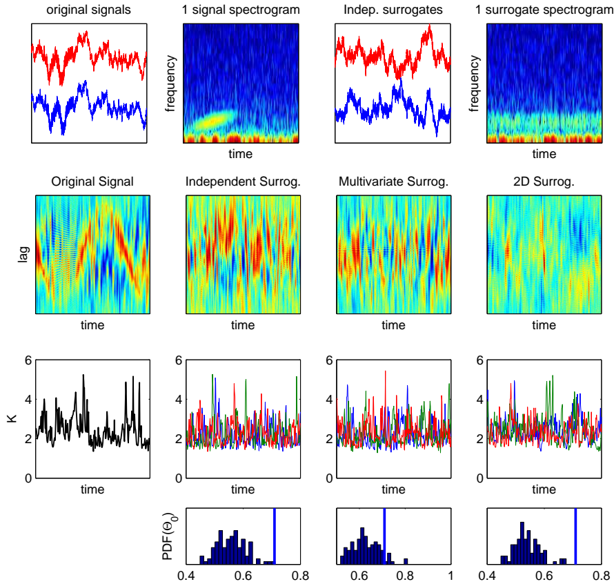
Figure 6. Nonstationary Cross-correlations. Top (from left to right): original signals with non-zero cross-correlation (displayed underneath: mainly a time-varying sinusoidal delay), the spectrogram of one of them, two independent surrogates and the spectrogram of one of them. Second line: cross-correlations of original surrogate and of surrogates (independent, multivariate or in time-lag domain from left to right). Third line: local contrast (measured here with Kurtosis of the difference between the estimate of the cross-correlation and the time-averaged one). Bottom: PDF of the test statistics \Theta_0 from the different versions of surrogates, and the statistics \Theta_1 for the original signals (vertical bar).
