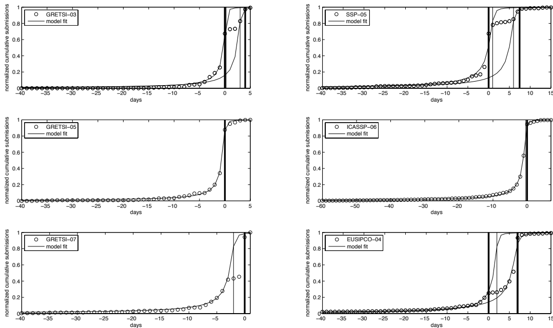
Fig. 3. Data and optimal least-squares model fits for all conferences. Actual (resp. fitted) deadlines are plotted as thick (resp. thin) vertical lines. In three cases (GRETSI-03, SSP-05 and EUSIPCO-04), the initial deadline has been officially extended, with an announcement a couple of days prior the initial deadline here referred to as T = 0 . In those cases, two models have been adjusted, with an estimated deadline fitted in the vicinity of each actual one. The corresponding values of the fitted parameters are reported in Table 1.
