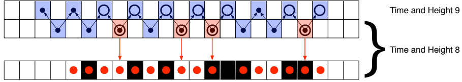
Fig. 5. Cells of \mathbb{T}^8 and \mathbb{T}^9 are colored in red and blue. Active cells are marked by a red dot. Red arrows link the sites of C^8 to their corresponding cells in c^8 . In this example, these cells are active in c^8 . Thus the correspondence criterion is verified at time 8.
