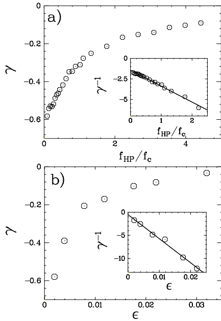
FIG. 4: a) The skewness \gamma of the fluctuations at \epsilon = 2 \cdot 10^{-3} is plotted as a function of f_{\text{HP}} . Inset: \gamma^{-1} is linear in f_{\text{HP}}/f_c . b) \gamma as a function of \epsilon . Inset: \gamma^{-1} is linear in \epsilon .
