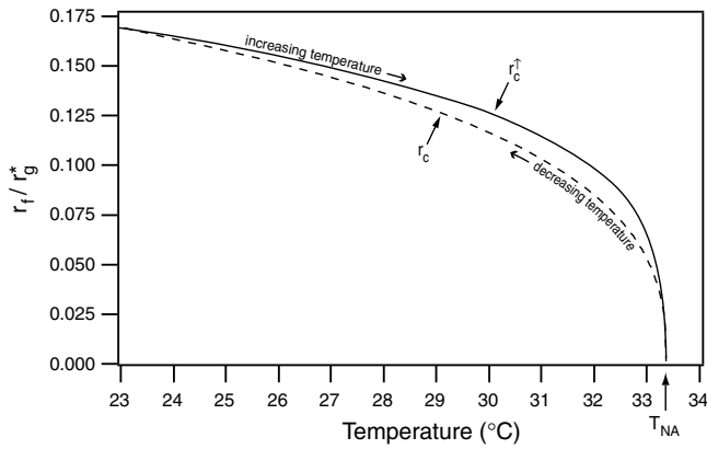
Fig. 8. Radius of the facet as a function of the temperature at increasing temperature (solid line, curve r_c^\uparrow ). For comparison, we reported the critical radius as a function of the temperature (dashed line, curve r_c ).
