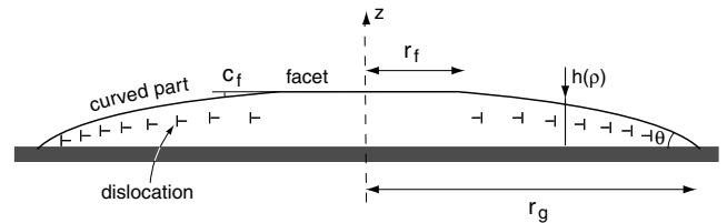
Fig. 2. Droplet configuration.
