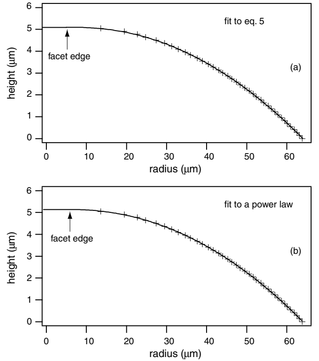
Fig. 7. a) Experimental profile (crosses) determined from the photograph shown in Figure 1. The solid line is the best fit to equation (5) with c_f = 0 . The arrow marks the facet edge given by the fit. The latter is pretty far from the last fringe detected experimentally. This shows all the difficulty to measure the facet radius (the top of the droplet is very flat). b) Same experimental data fitted to a power law. The size of the facet is found a bit larger than using the previous fit and the profile exponent is \nu = 2.1 .
