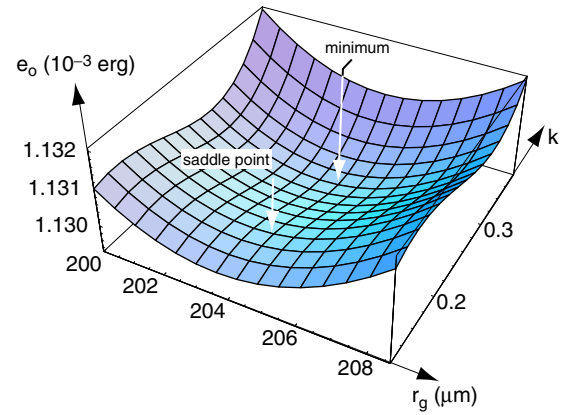
Fig. 4. 3D plot of the droplet energy e_o as a function of k = r_f/r_g and r_g . The saddle point and the absolute minimum are indicated by two arrows (8CB, T = 24^\circ\text{C} , V = 10^{-6} \text{ cm}^3 ).
