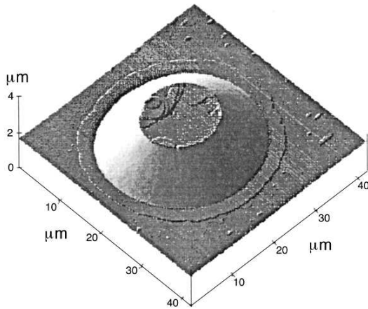
Fig. 14. Three-dimensional view of a droplet of the chiral liquid crystal XI/12 obtained by tapping mode atomic force microscopy. The droplet has been deposited in the smectic A phase at high temperature (about 100 °C) and then slowly cooled down to the room temperature in the SmC* phase (from Ref. [33]).
