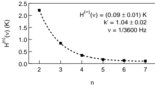
Fig. 8. Amplitude H^{(n)} vs. bead position n .
