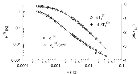
Fig. 4. Experimental H^{(2)} and \theta^{(2)} vs. frequency \nu .
