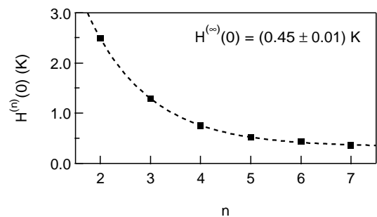
Fig. 7. Experimental H^{(n)}(0) vs. bead position n . We observe that the temperature difference at zero frequency between the bead n and the atmosphere decreases almost exponentially when n increases but does not vanish far away from the heat source (large n ).
