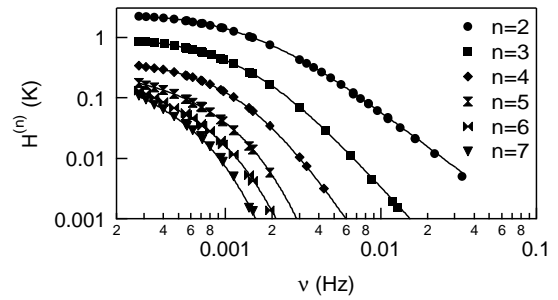
Fig. 5. Amplitude H^{(n)} vs. frequency \nu . The amplitude H^{(n)} decreases faster with increasing frequency \nu for larger n ( F = 100 N, dry contacts, the lines are only guides for the eye).
