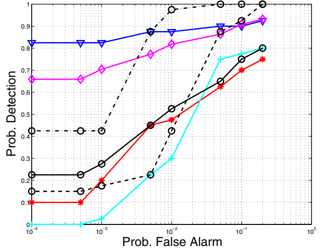
Figure 3. DETECTION VS. FALSE ALARM RATES. T = 1\text{min} . For distance D_\alpha and for attacks #3(7%,*), 4(12%, \nabla ), 6(10%,+), 7(27%, \diamond ), 8(4%,o) in Table 1. For 8(4%,o), dashed and mixed lines correspond to K_{\Delta}^{1d} , with \Delta = 10\text{ms} and \Delta = 40\text{ms} , for comparison.
