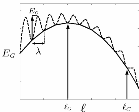
FIG. 3: Sketch of the Griffith potential energy E_G as a function of crack length \ell with constant applied stress (solid line). The energy barriers E_C and the discretization scale \lambda are represented by the dashed curve.
