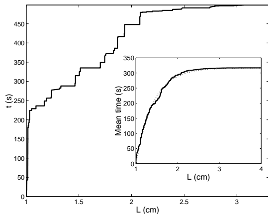
FIG. 1: Time versus crack length for a single experiment showing crack jumps and crack arrest. In insert, average time to reach L (10 experiments with F = 270\text{N} and L_i = 1\text{cm} ). The dotted curve is obtained from integration of eq.(1) [9].
