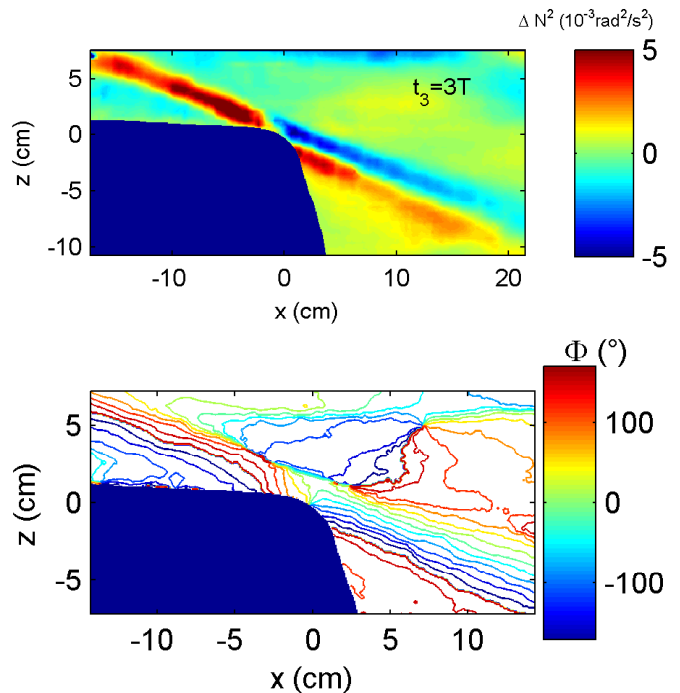
FIG. 2: (Color online) Panel a presents the two-dimensional vertical density gradient, while panel b shows the phase. Both plots have been averaged over one tidal period of the experiment around t = 3T . Horizontal and vertical distances are in cm. The generation point C appears to be an amphidromic point around which the phase of the wave rotates.
