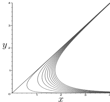
FIGURE 2: \rho = xy(x^2 - y^2) for various values of \rho .
