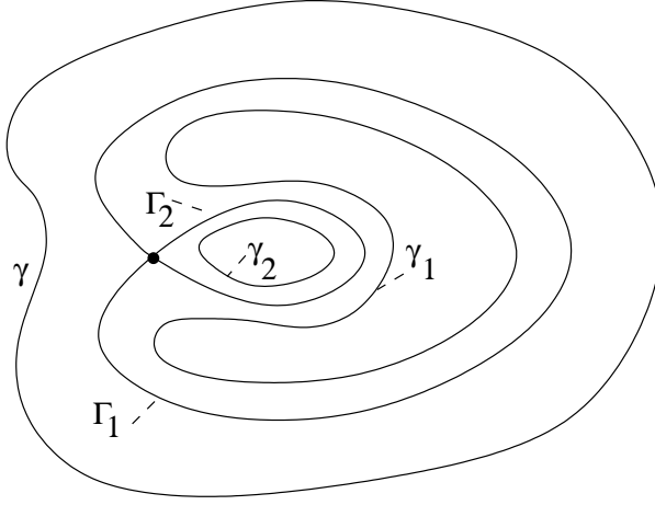
Figure 7: One separatrix loop inside the other.
