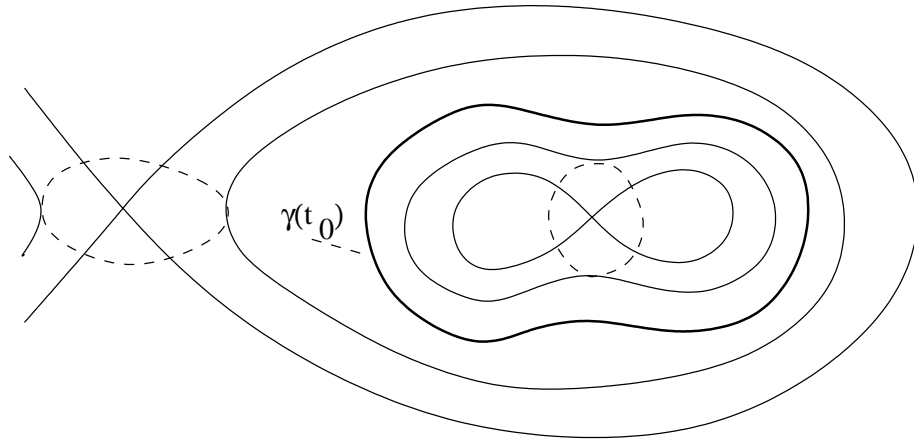
Figure 4: Local vanishing cycles having nonzero intersection index with the ovals of the family that contains \gamma(t_0) .
