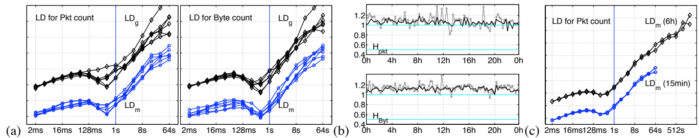
Fig. 8. One day: Statistics (Jp2US). (a) LDs for 15min long traces (Left: Pkt; Right: Byte): Global (black \diamond ) and median-sketch (blue \bullet ). (b) Estimates for H vs. time: Global (gray), median-sketch (black). (c) LDs for 6h-long traces (Jp2US): Average LD over 15-min long traces (blue \bullet ) and LD computed fully on 6h trace (black \diamond ).
