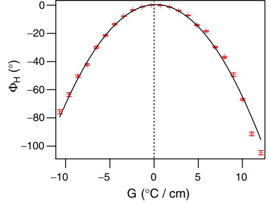
Fig. 1: Phase shift as a function of the temperature gradient ( d = 100 \mu\text{m} , homeotropic anchoring).
